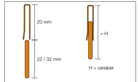
Schlüter®-SHOWERPROFILE-R
